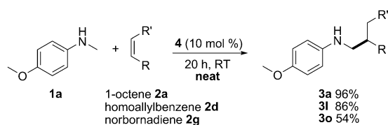
Scheme 4. Solvent-free hydroaminoalkylation.
